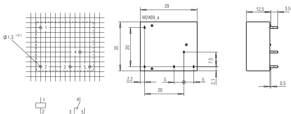
OA 5671 10 mm Pinabstand
