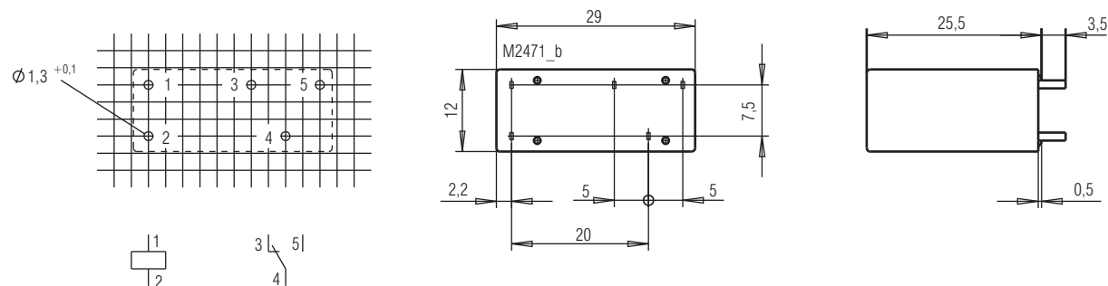
OA 5672 10 mm Pinabstand
